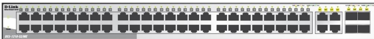
Figure 1.1 – DES-1210-52/ME Front Panel
