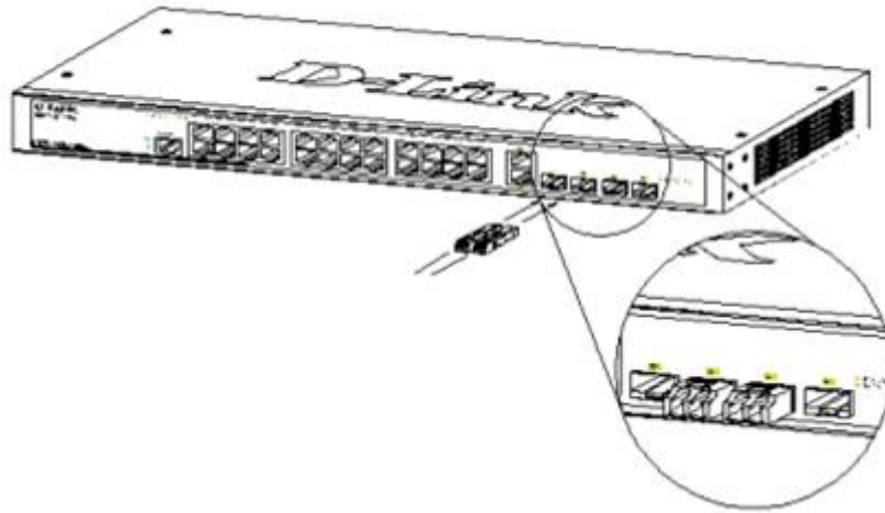
Figure 1.5 - Inserting the SFP modules into the Switch
