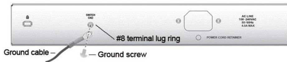
Figure 2.6 – Connect a Grounding Cable
